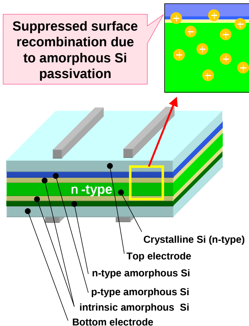
HIT solar cell
