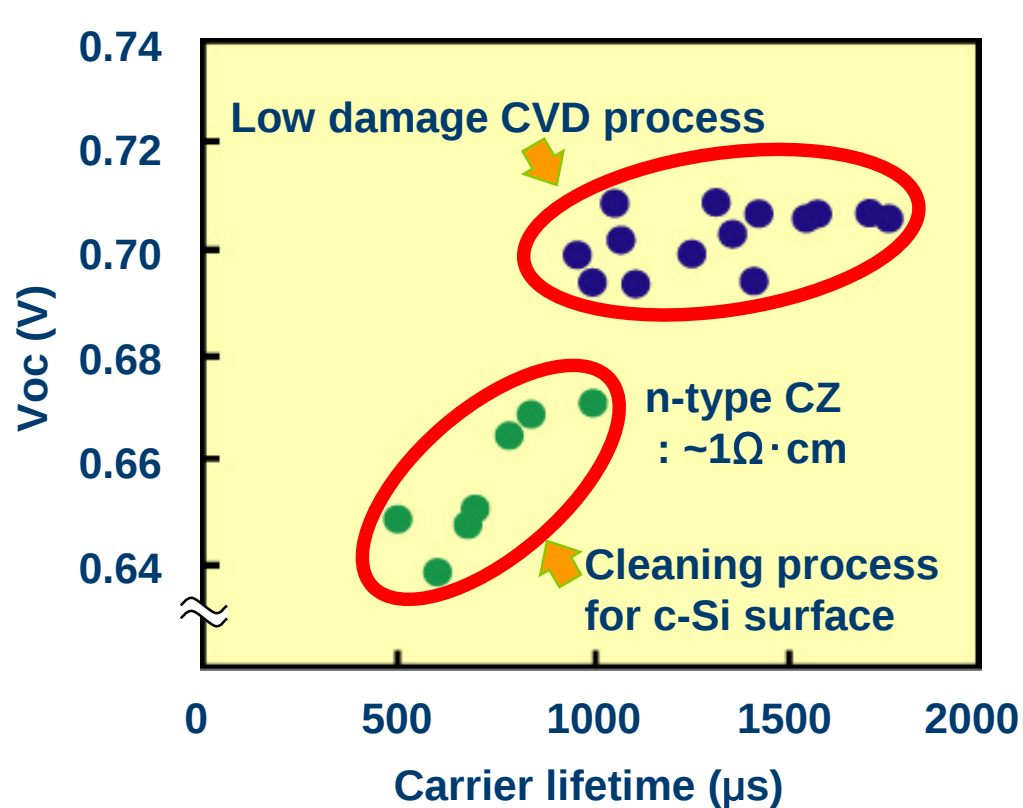
Relationship between carrier lifetime (μ-PCD) and Voc
