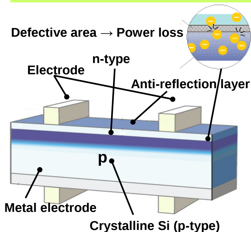
Conventional c-Si solar cell
