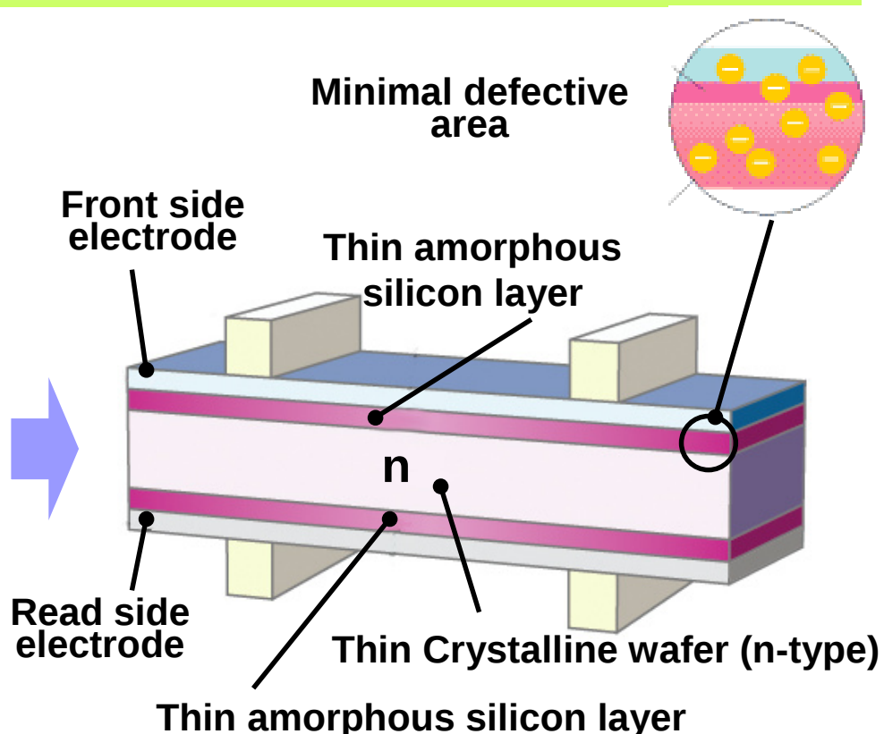
HIT solar cell
