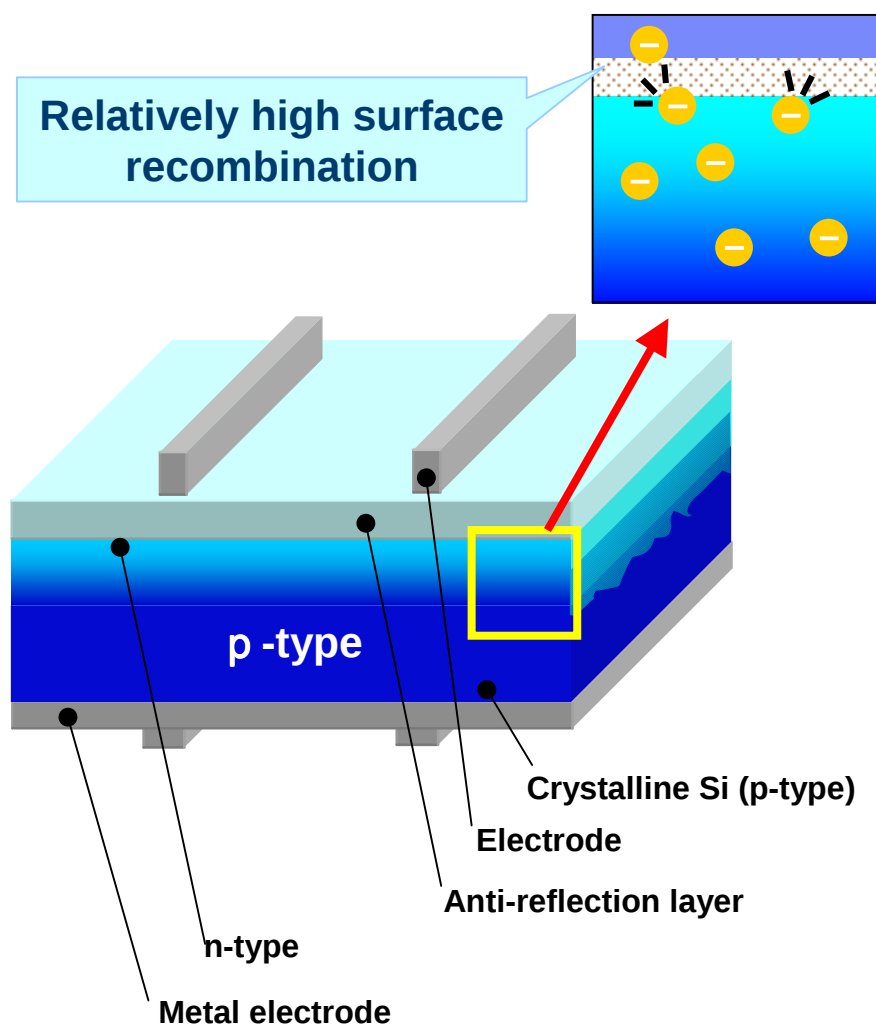
Conventional c-Si solar cell
